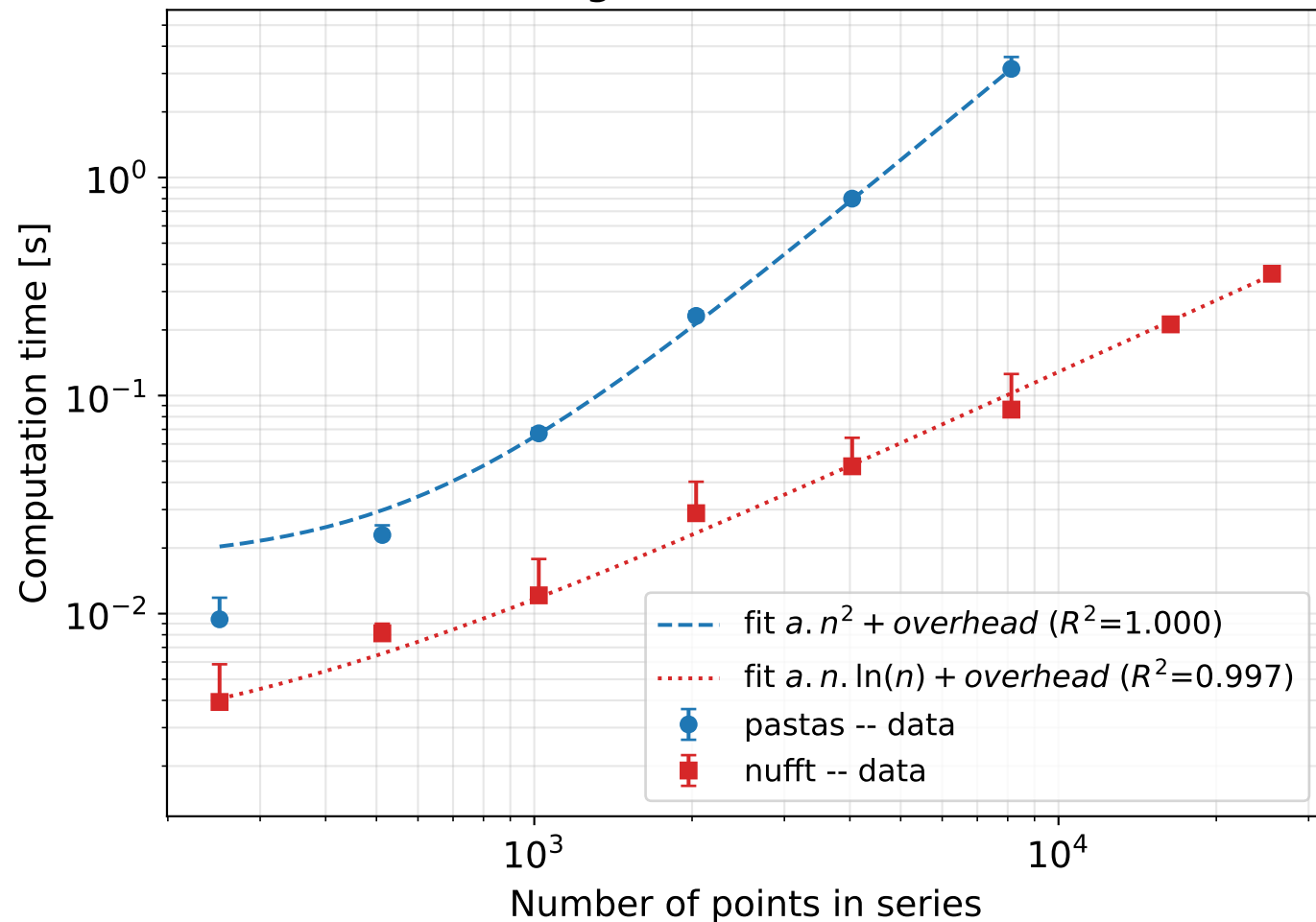
gaussian kernel
